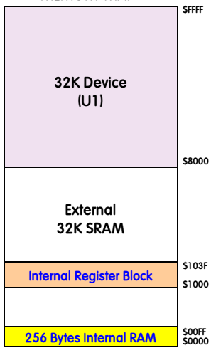
MEMORY MAP*
